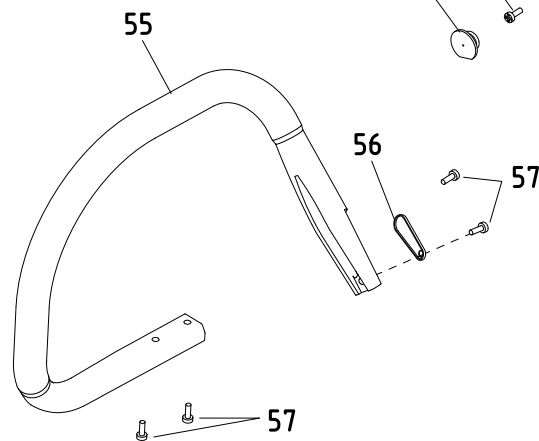
TCS3800/TCS4100 base unit (easy start)
